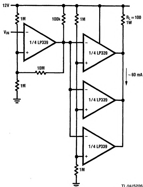
Comparator With 60 mA Sink Capability
