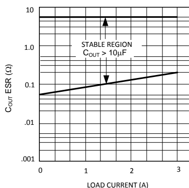
Figure 3. ESR Curve
