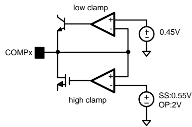
Figure 4. Error Flag Operation
