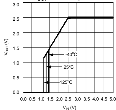
V_{IN} vs V_{OUT} Over Temperature
