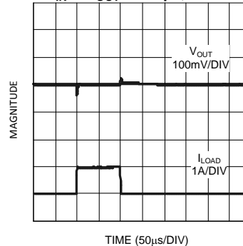
Load Transient Response C_{IN} = C_{OUT} = 100\mu\text{F} , POSCAP
