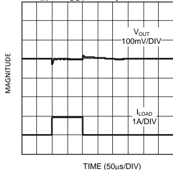
Load Transient Response C_{IN} = C_{OUT} = 100\mu\text{F} , OSCON
