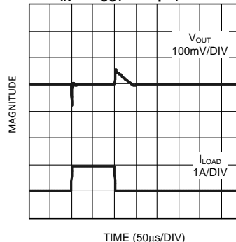
Load Transient Response C_{IN} = C_{OUT} = 10\mu\text{F} , OSCON
