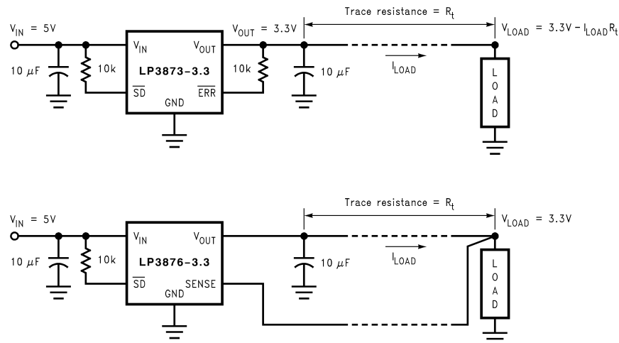
Figure 5. Improving remote load regulation using LP3876
