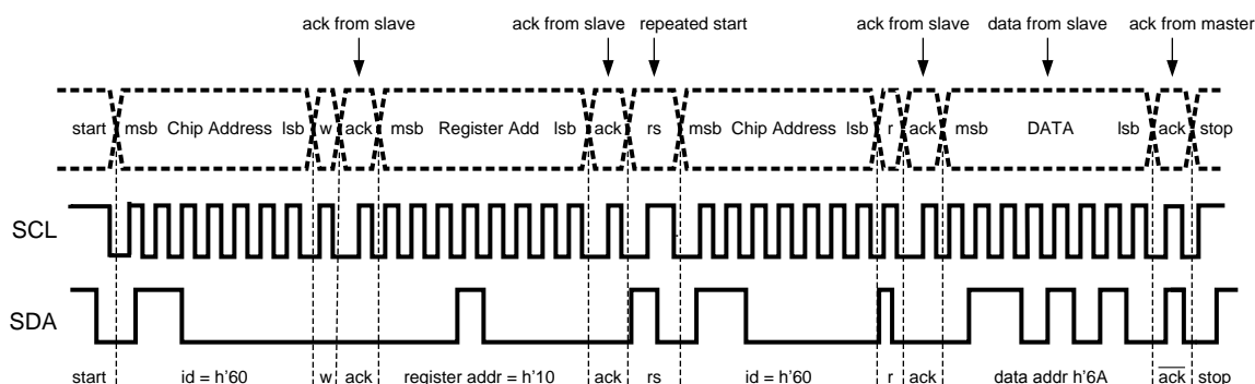
Figure 19. I²C Read Cycle
