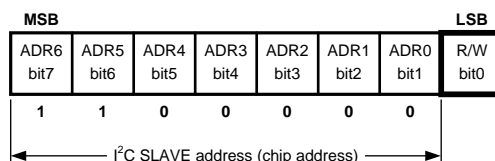
Figure 17. I²C Chip Address (see note above)
