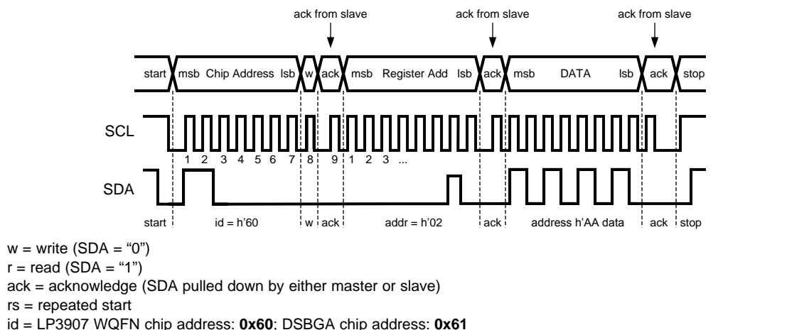
Figure 18. I²C Write Cycle
