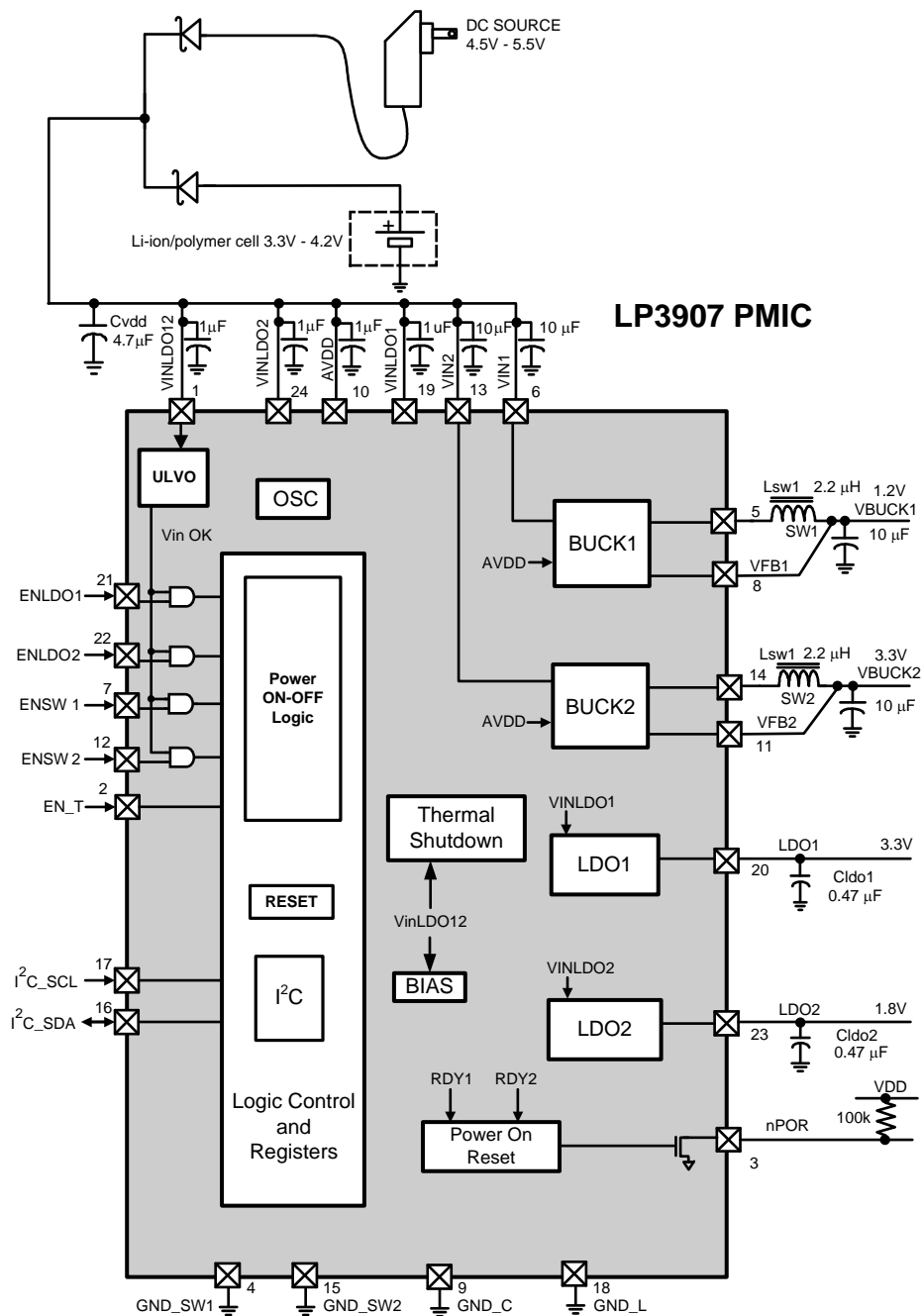
Application Circuit
