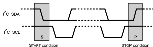
Figure 16. START and STOP Conditions
