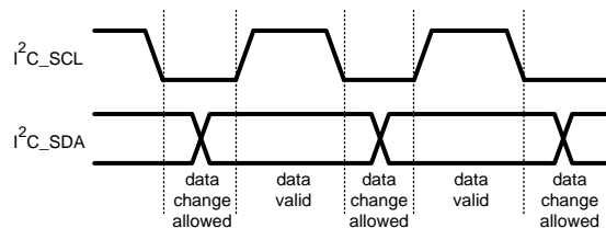
Figure 15. I²C Signals: Data Validity
