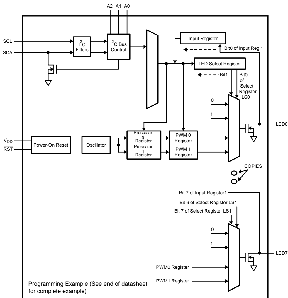
Figure 2. For Explanation of LP3944 Operation, Please Refer to Theory of Operation in Application Notes.
