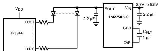
Figure 13. Application Circuit
