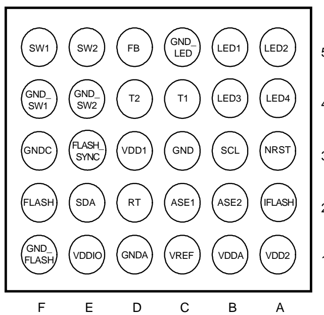
Figure 3. Top View
