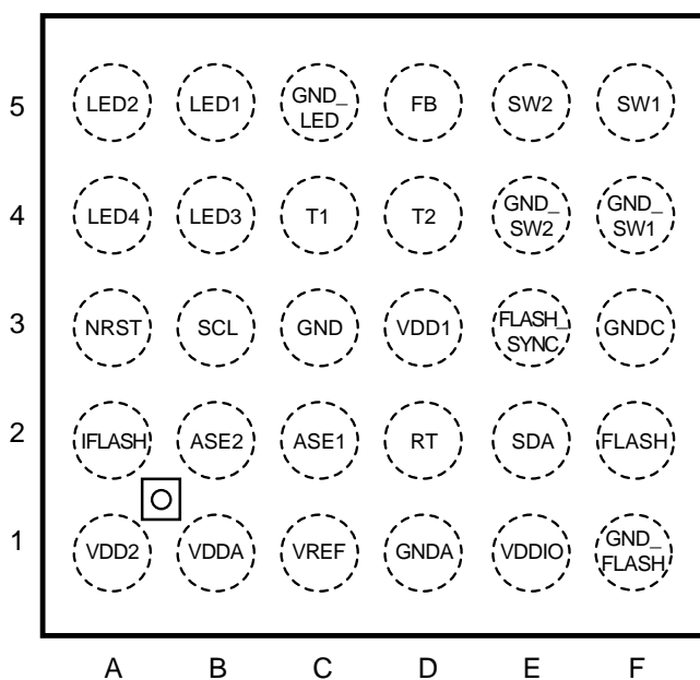
Figure 2. Top View
