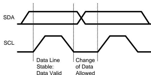
Figure 17. Bit Transfer
