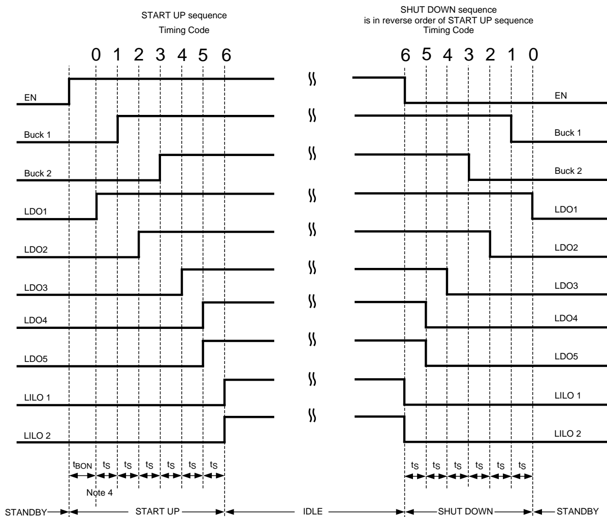
Figure 14. LP8725-E Startup and Shutdown Sequence if CONFIG=GND, DEFSEL=VIN1 or GND Note 1, Note 2
