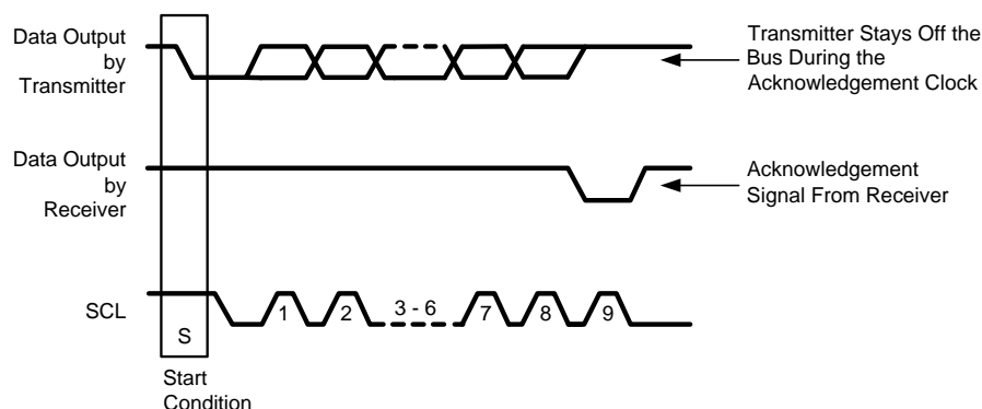
Figure 19. Bus Acknowledge Cycle
