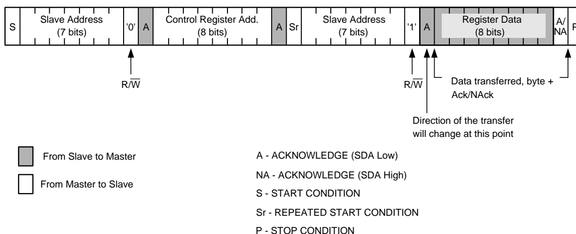
Figure 21. Register Read Format
