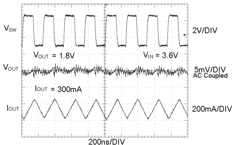
Figure 15. Typical PWM Operation
