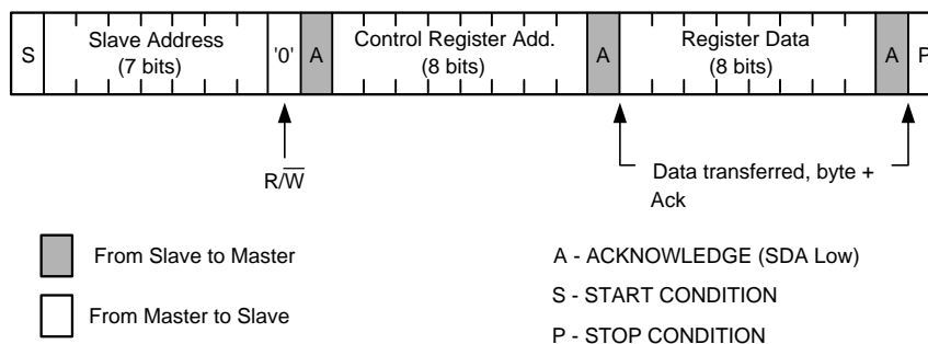
Figure 20. Register Write Format
