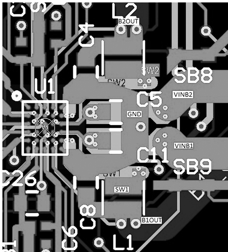
Figure 22. Layout Scheme used on Eval Board
