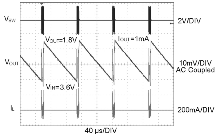
Figure 16. Typical ECO Operation
