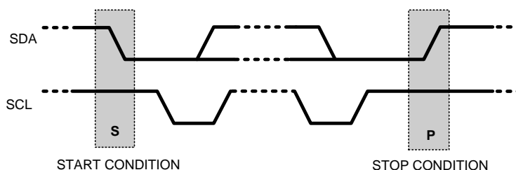
Figure 18. Start and Stop Conditions
