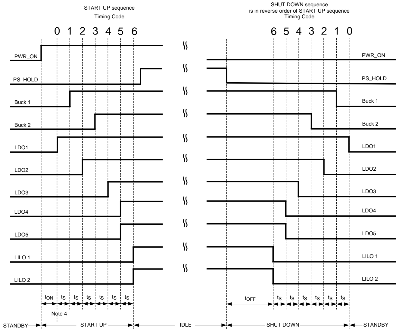
Figure 13. LP8725-E Startup and Shutdown Sequence if CONFIG=VIN, DEFSEL=VIN1 or DEFSEL=GND Note 1, Note 2
