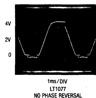
Voltage Follower with Input Exceeding the Negative Common-Mode Range ( V_S = 5V, 0V )
