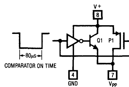
Figure 3. V_{PP} Output Switch
