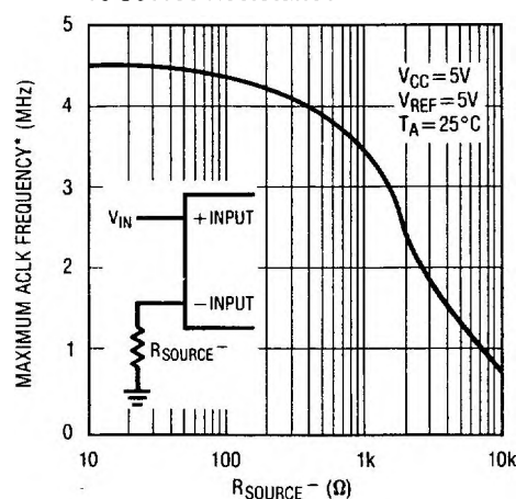
Maximum Conversion Clock Rate vs Source Resistance
