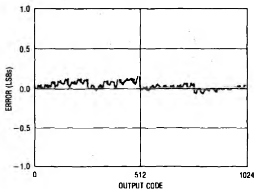
Linearity Plot
