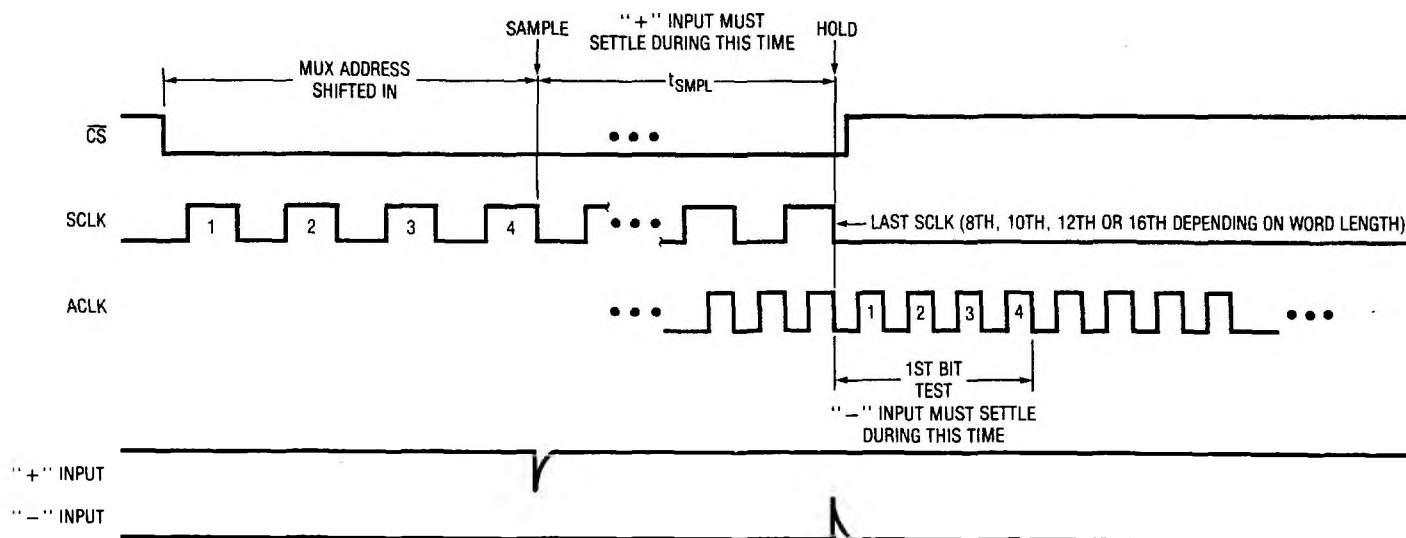
Figure 10. “+” and “-” Input Settling Windows
