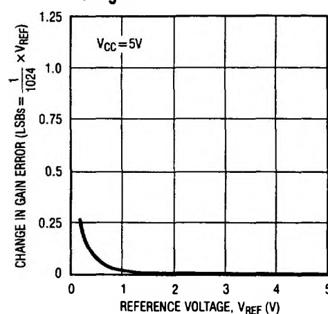
Change in Gain Error vs Reference Voltage
