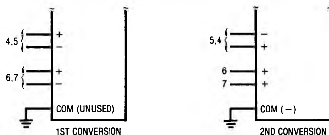
Figure 1. Examples of Multiplexer Options on the LTC1090
