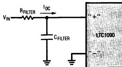
Figure 13. RC Input Filtering
