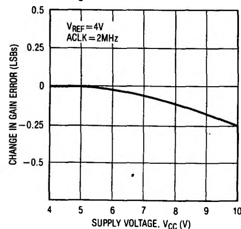
Change in Gain Error vs Supply Voltage
