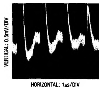
Figure 16. Poor Reference Settling Can Cause A/D Errors
