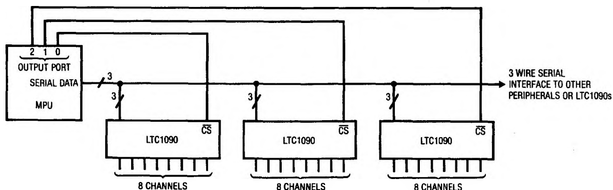
Figure 5. Several LTC1090s Sharing One 3 Wire Serial Interface
