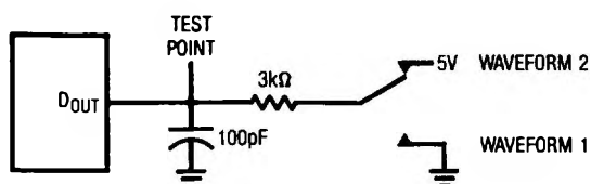
Load Circuit for t_{dis} and t_{en}
