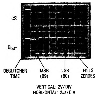
Scope Trace of LTC1090 "Quick Look" Circuit Showing A/D Output of 01010101 (155 HEX )
