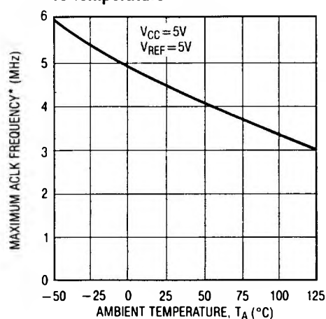
Maximum Conversion Clock Rate vs Temperature
