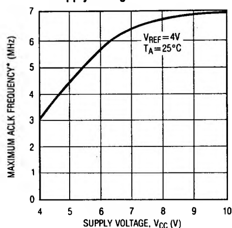
Maximum Conversion Clock Rate vs Supply Voltage
