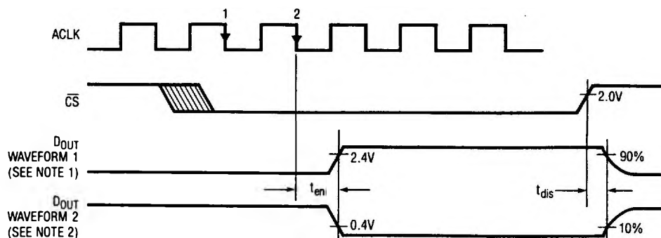
Voltage Waveforms for t_{en} and t_{dis}
