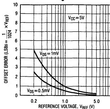
Unadjusted Offset Error vs Reference Voltage
