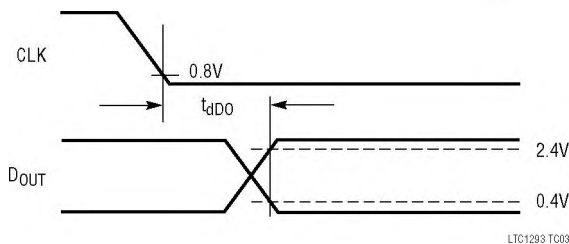
Voltage Waveform for D_{OUT} Delay Time, t_{dDQ}
