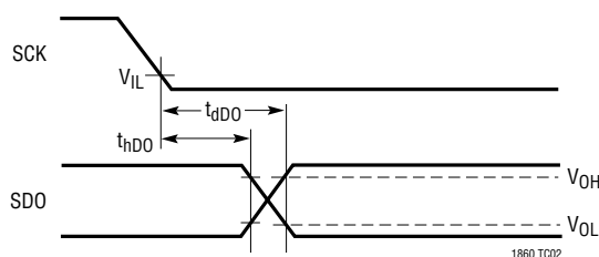
Voltage Waveforms for SDO Delay Time, t_{dDO}
