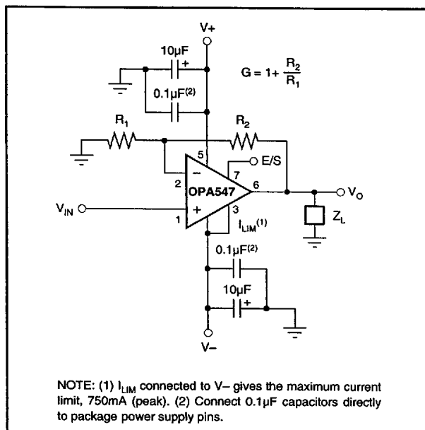
FIGURE 1. Basic Circuit Connections.
