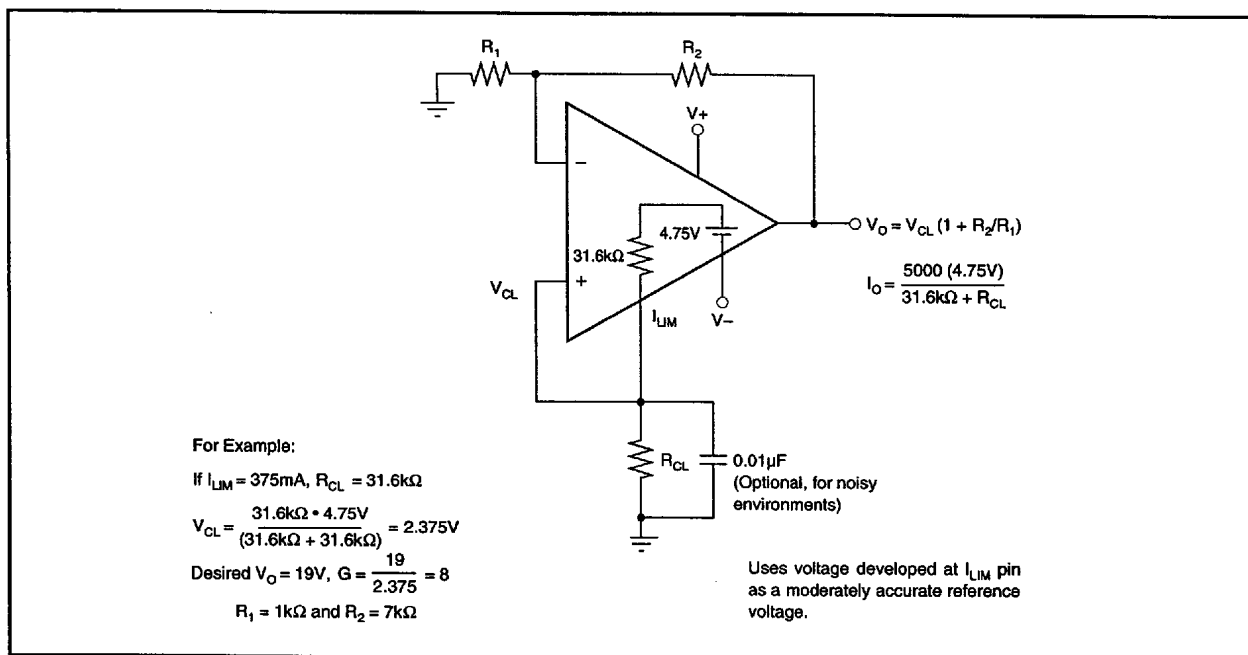
FIGURE 12. Voltage Source.
