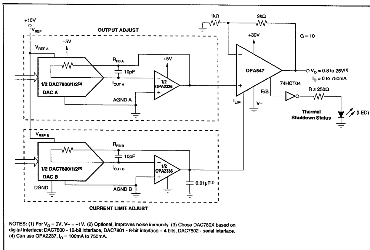
FIGURE 14. Digitally-Controlled Programmable Power Supply.
