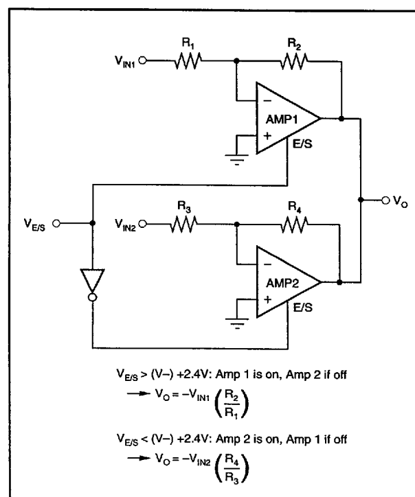
FIGURE 15. Swap Amplifier.
