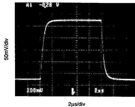
SMALL SIGNAL STEP RESPONSE G = 3 , C_L = 1000pF
