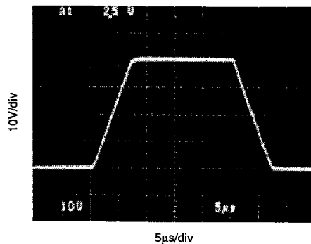
LARGE SIGNAL STEP RESPONSE G = 3 , C_L = 100pF , R_L = 50\Omega
