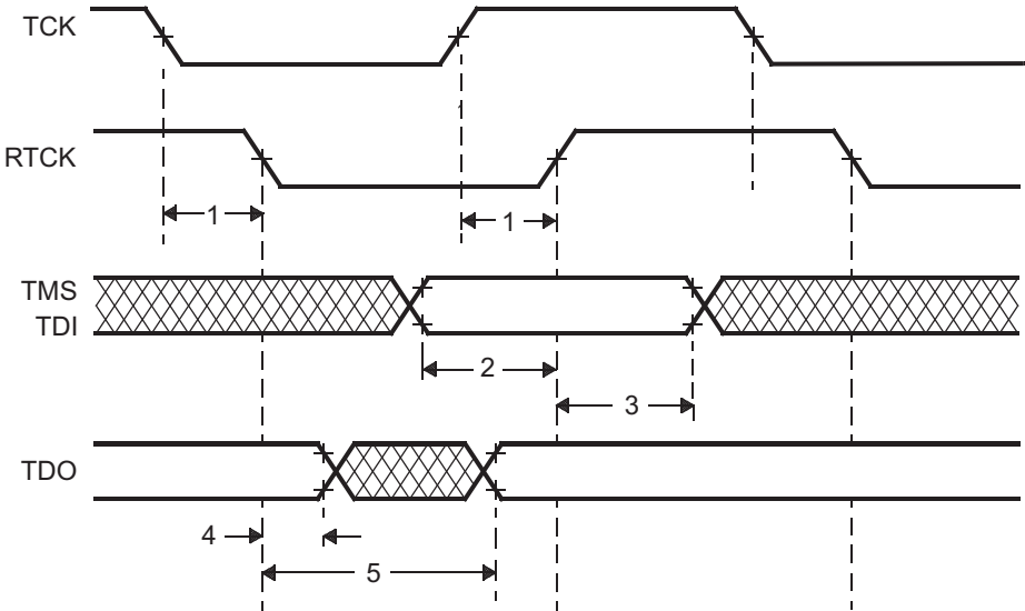
Figure 4-21. JTAG Timing
