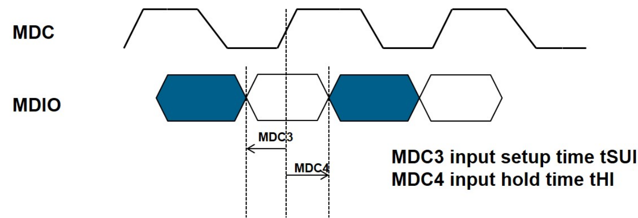
Figure 41. MDIO input timing
