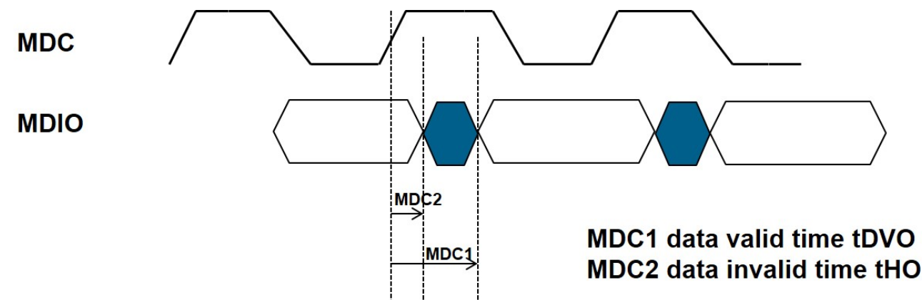
Figure 41. MDIO input timing
