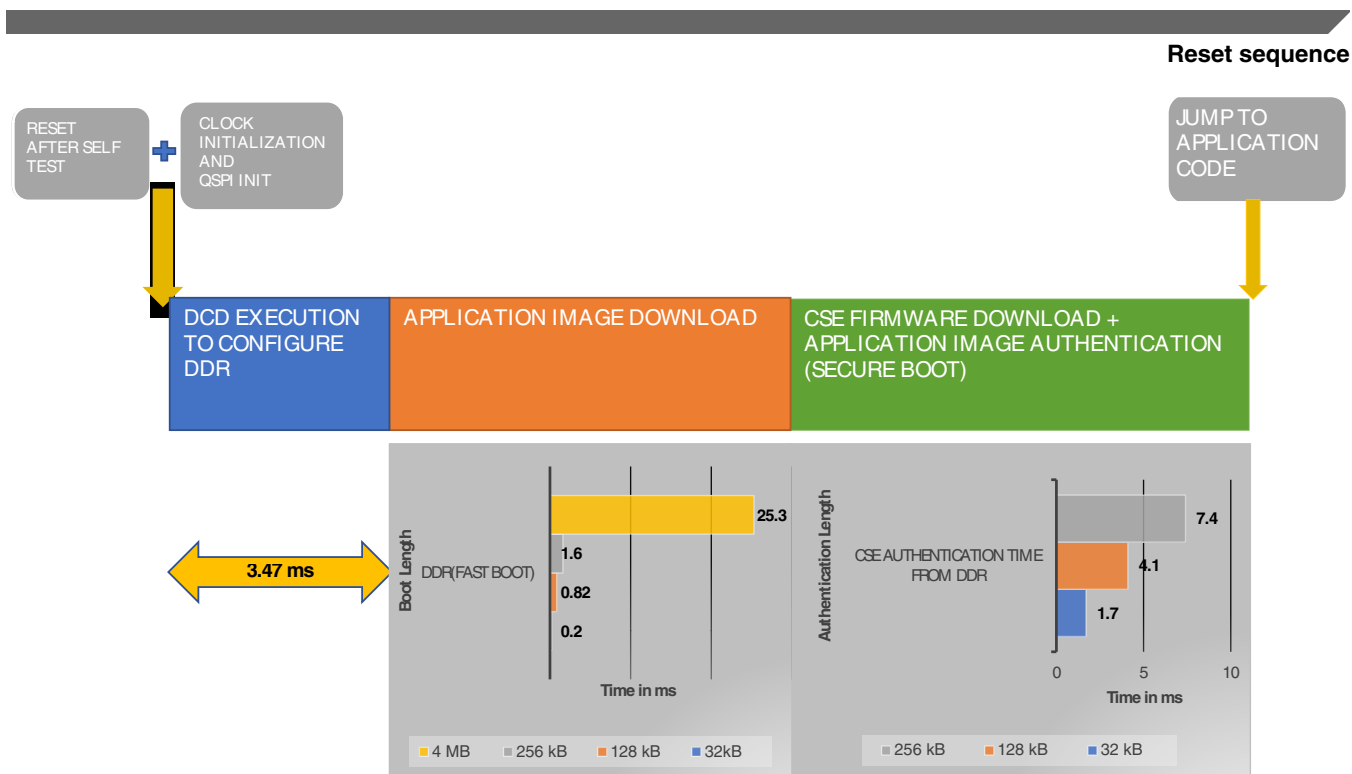
Figure 58. Boot diagram
