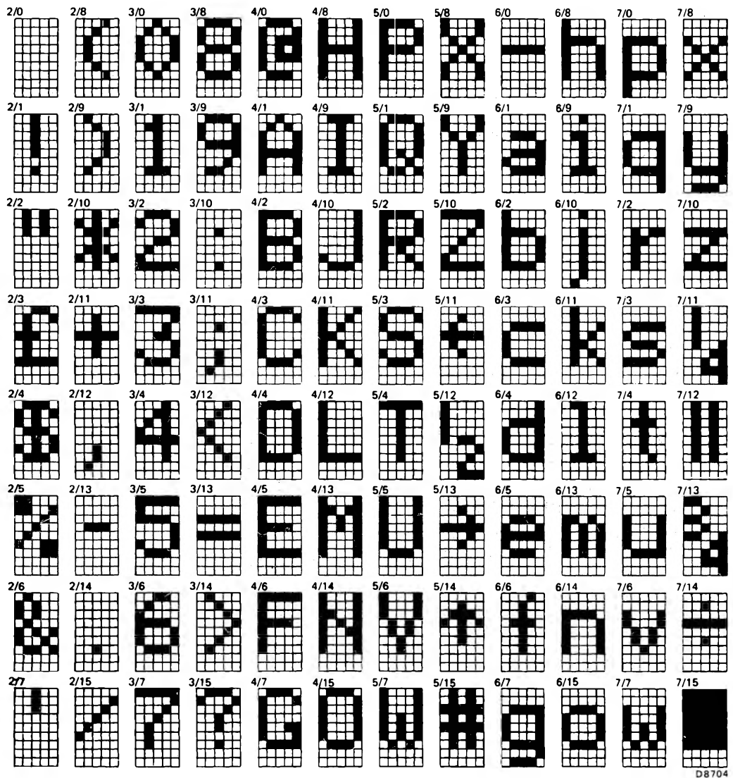
Fig. 11 SAA5050 character set (English).
