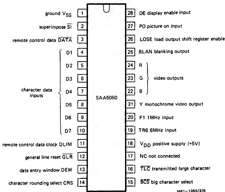
Fig.2 Pinning diagram
