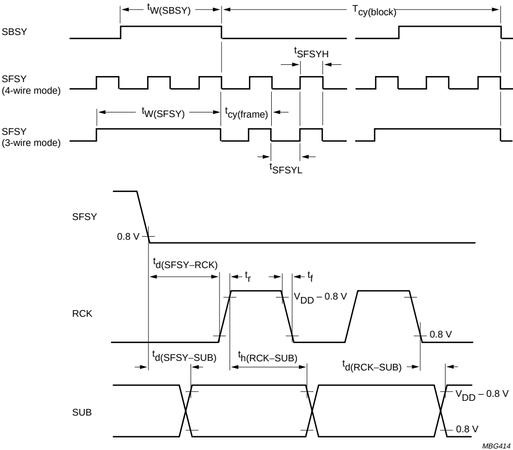
Fig.31 Subcode interface timing diagram.
