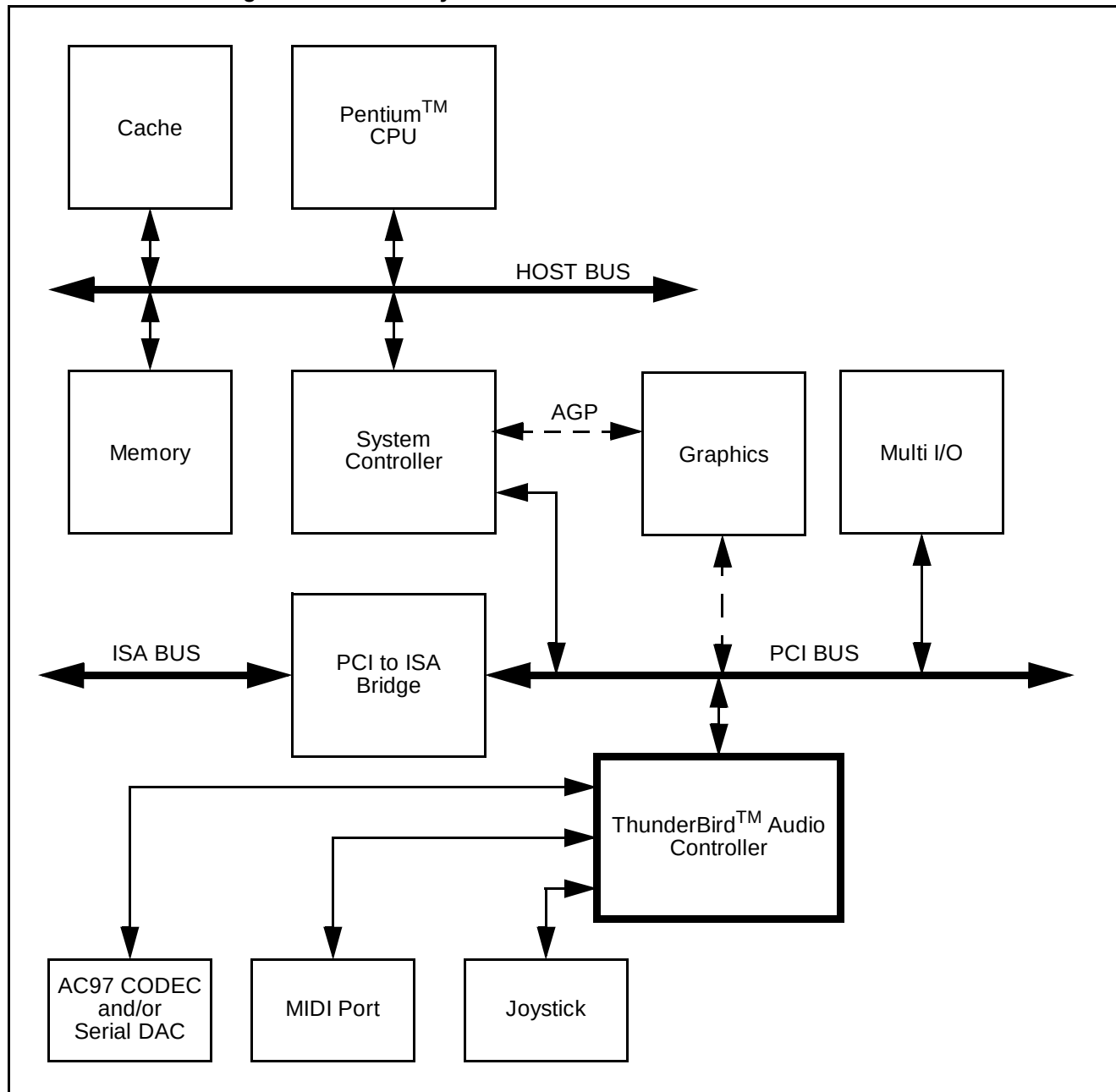
FIGURE 3 Block Diagram of a PC/AT System with the SAA7780
