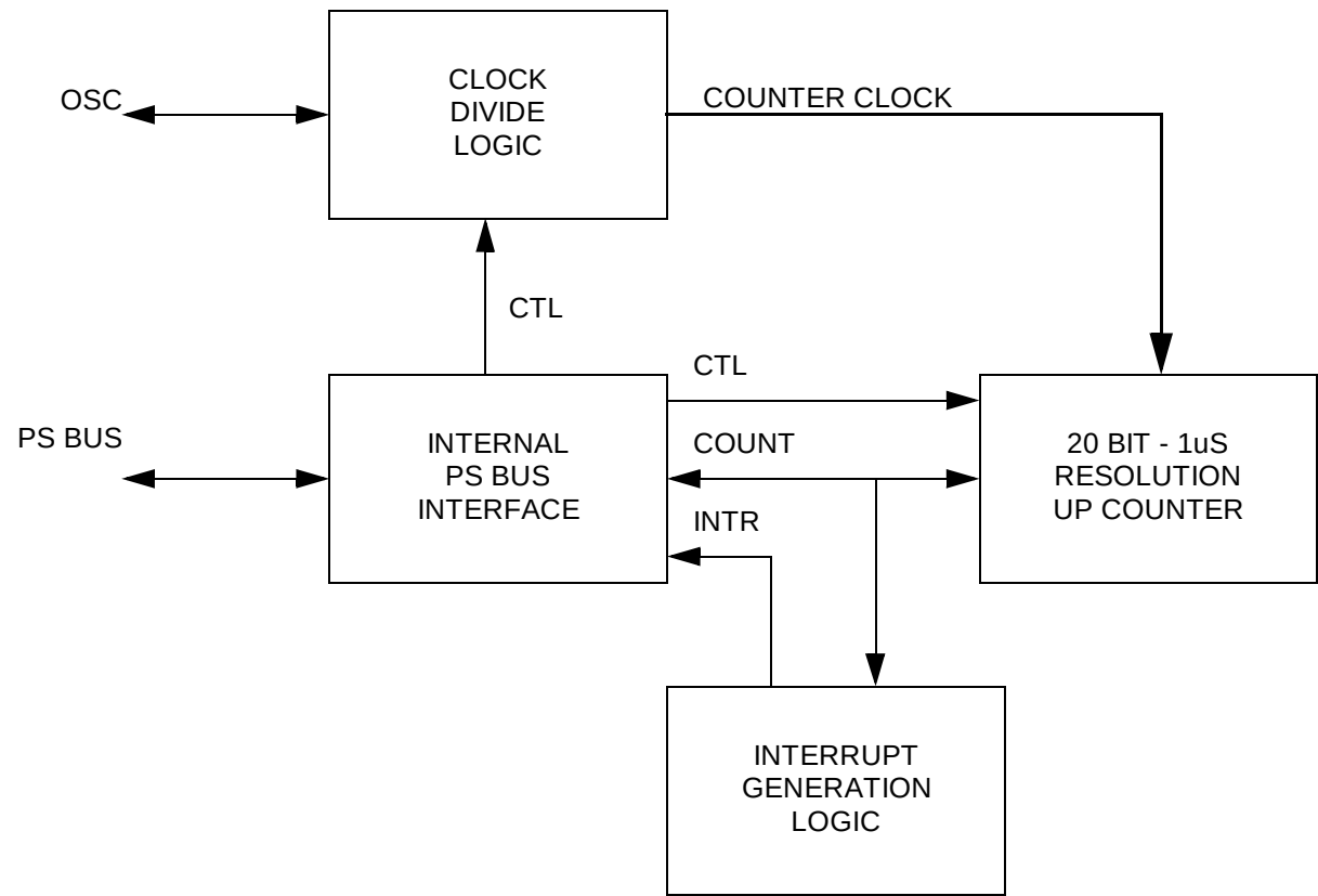
FIGURE 6 Multimedia Timer Block Diagram
