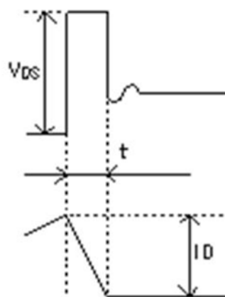
Waveforms during avalanche breakdown
