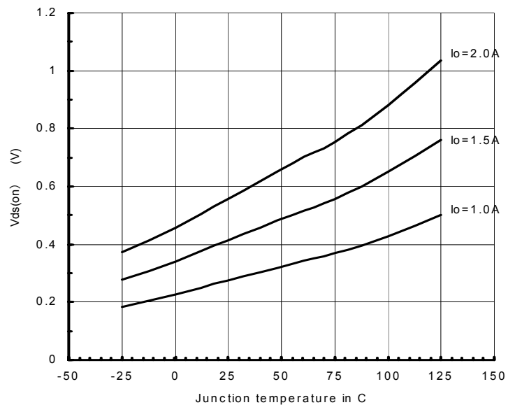
Normalized FET on resistance
