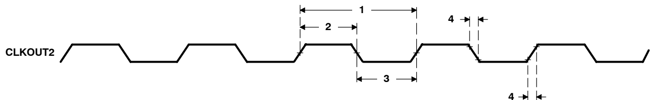
Figure 11. CLKOUT2 Timings
