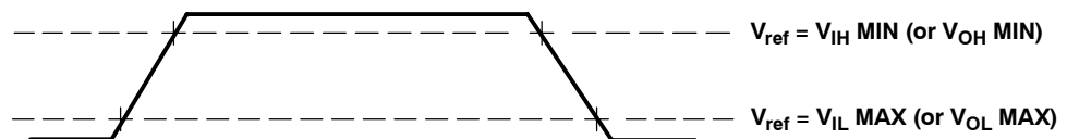
Figure 8. Rise and Fall Transition Time Voltage Reference Levels
