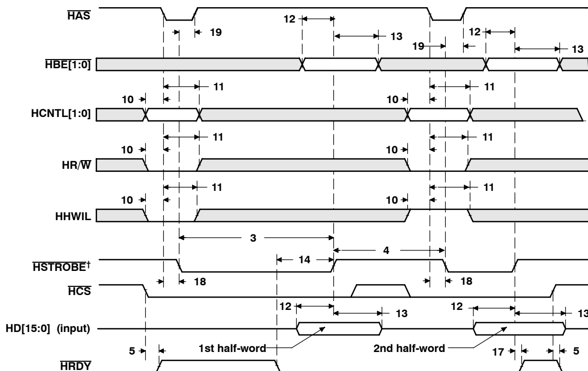
Figure 31. HPI Write Timing ( \overline{\text{HAS}} Used)
