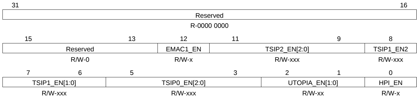
Figure 3-1. Device Control Register (DEVCTL)
