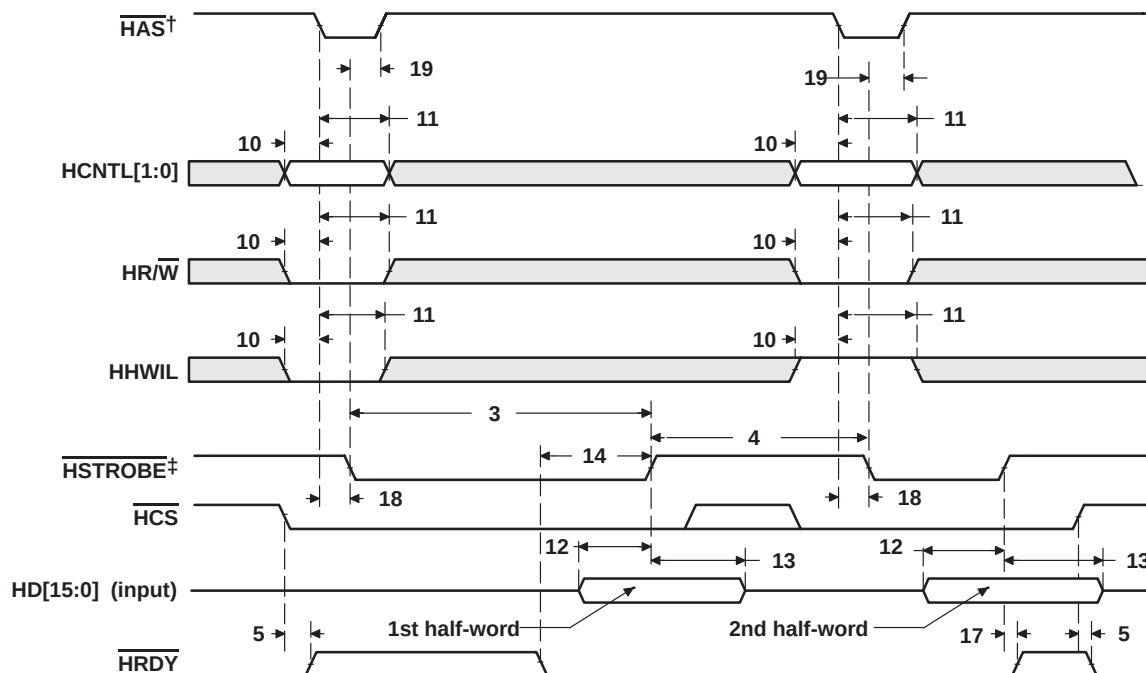
Figure 49. HPI Write Timing ( \overline{HAS} Used)
