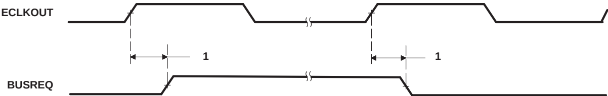
Figure 42. BUSREQ Timing
