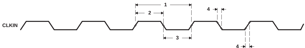
Figure 23. CLKIN Timings
