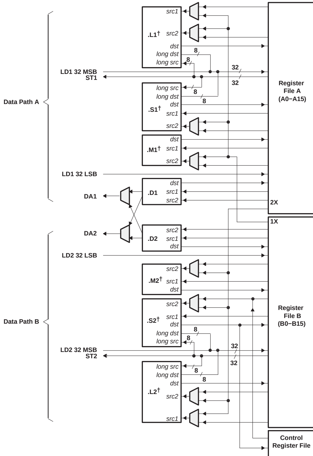
Figure 1. 320C67x™ CPU (DSP Core) Data Paths
