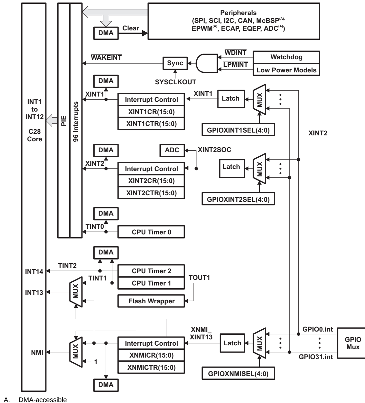
Figure 3-3. External and PIE Interrupt Sources
