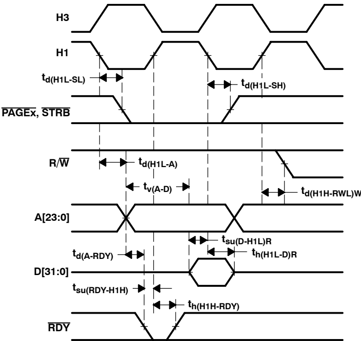
Figure 20. Timing for Memory ( \overline{\text{STRB}} = 0 and \overline{\text{PAGE}} = 0 ) Read
