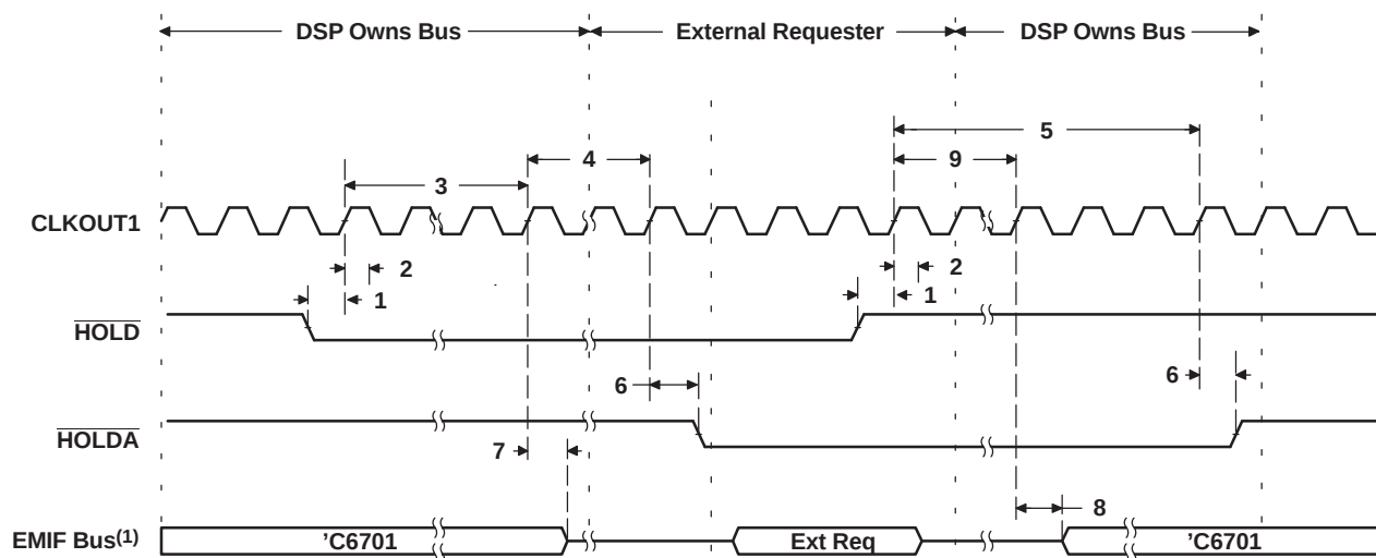
Figure 24. \overline{HOLD}/\overline{HOLDA} Timing
