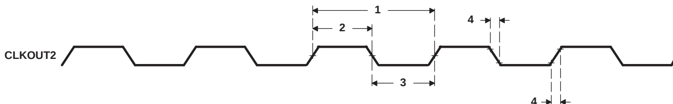
Figure 10. CLKOUT2 Timing
