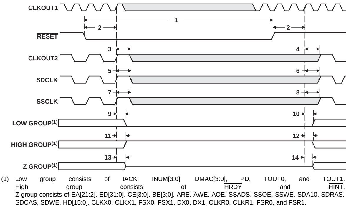
Figure 25. Reset Timing
