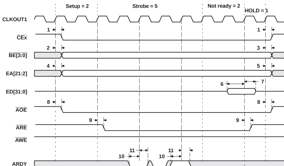
Figure 12. Asynchronous Memory Read Timing
