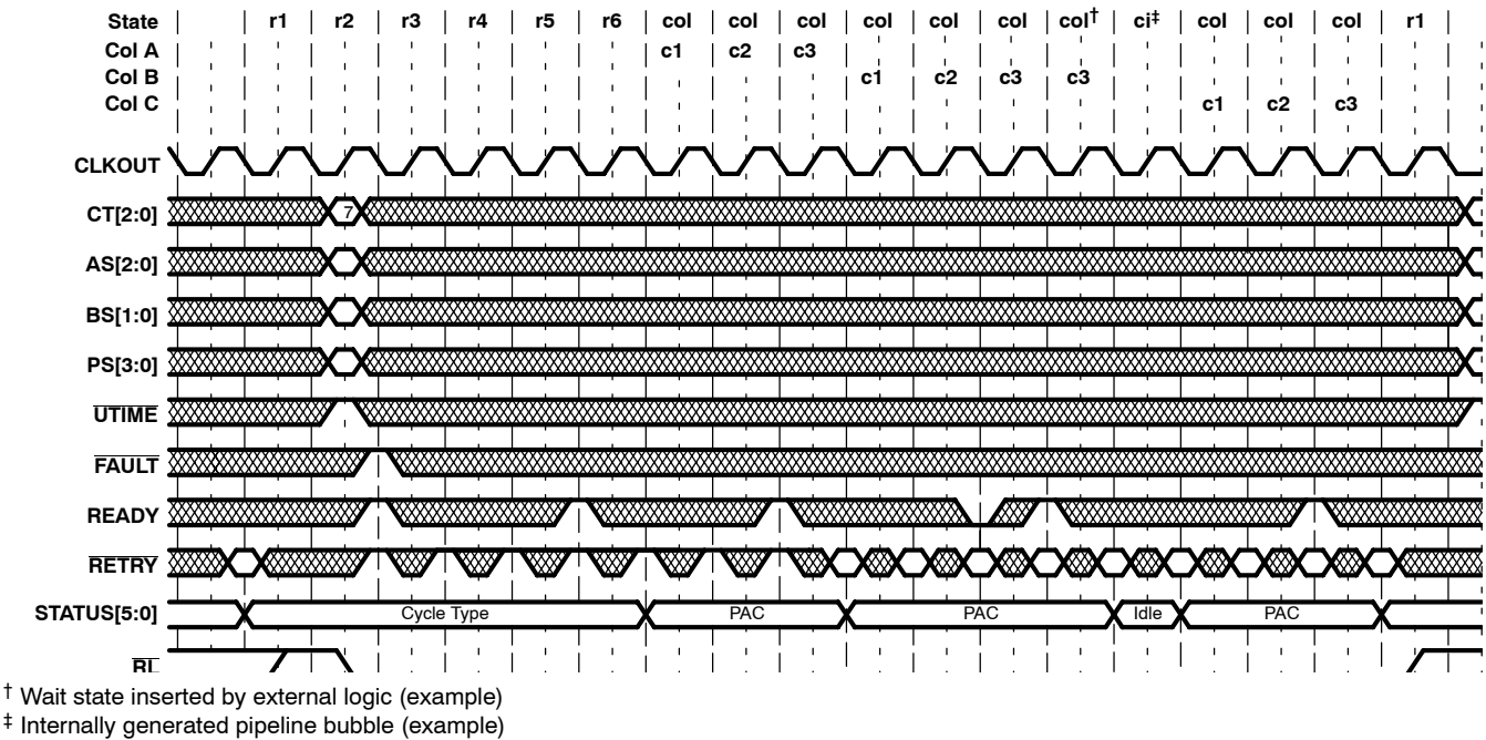
Figure 73. 3-Cycle/Column Block-Write-Cycle Timing
