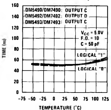
Transition Time to Outputs C &amp; D
