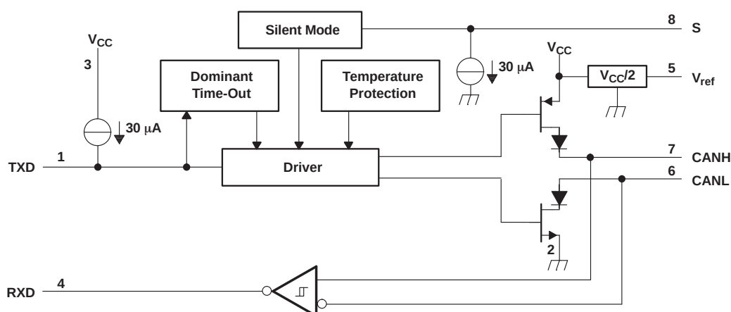
FUNCTION BLOCK DIAGRAM
