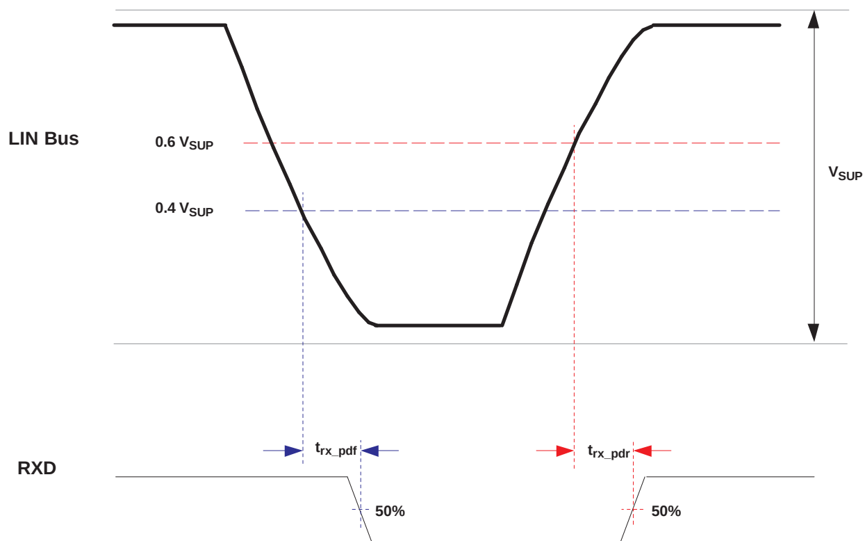
Figure 9. Propagation Delay
