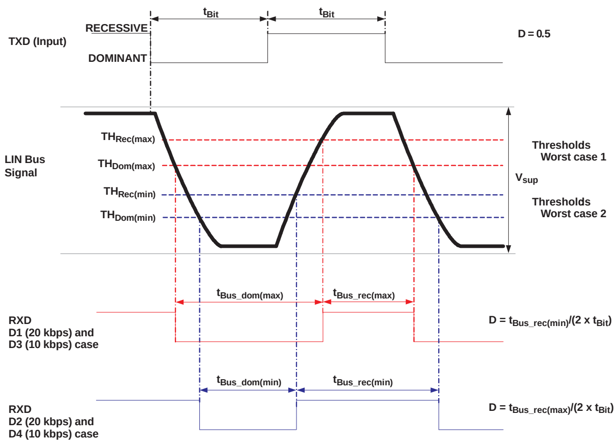
Figure 8. Definition of Bus Timing Parameters
