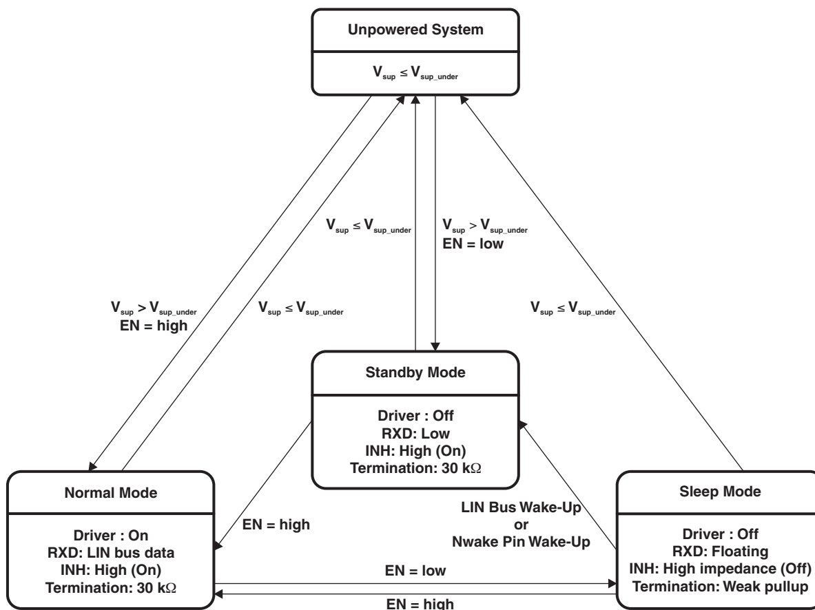
Figure 2. Operating States Diagram
