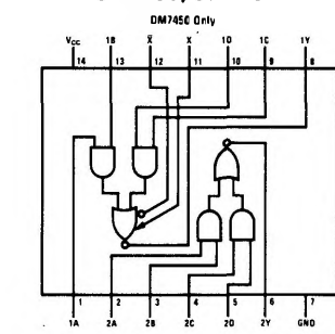
DM7450, DM7451
