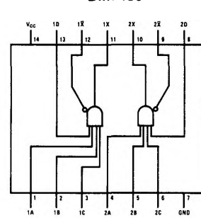
DM7460
