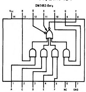
DM7453, DM7454
