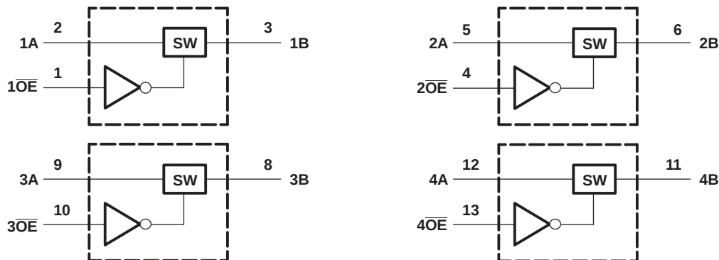
Figure 2. SIMPLIFIED SCHEMATIC, EACH FET SWITCH (SW)
