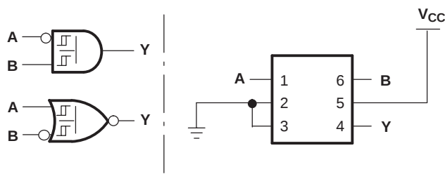
Figure 3. 2-Input AND Gate With Inverted A Input
