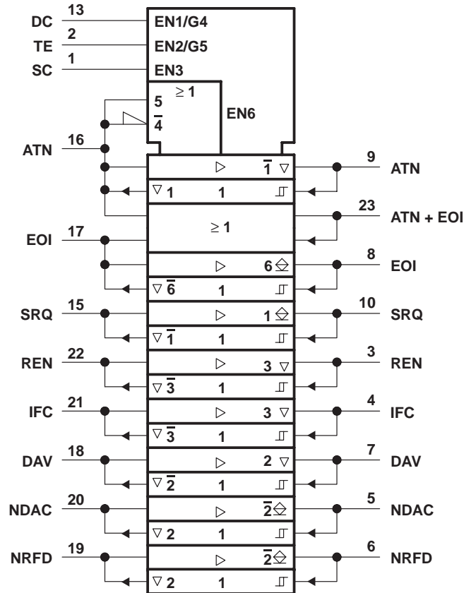
logic symbol†
