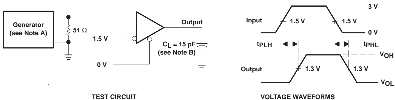
TEST CIRCUIT
