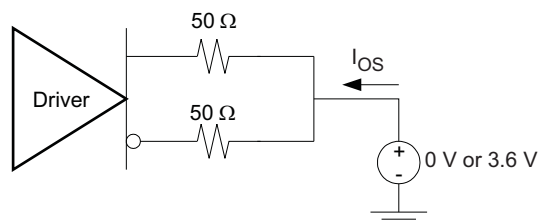
Figure 23. TMDs Main Link Short Circuit Output Circuit
