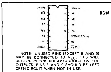
Fig. 1 Pin connections (top)
