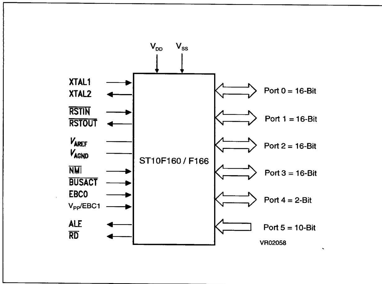
Figure 1. Logic Symbol
