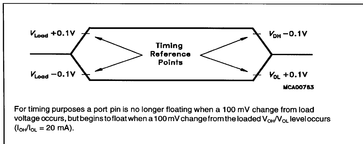
Figure 12. Float Waveforms
