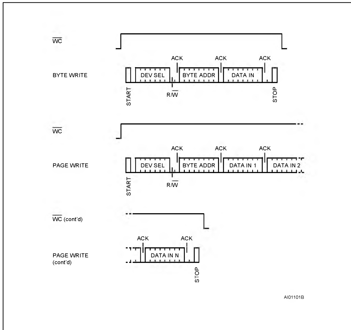
Figure 9. Write Modes Sequence with Write Control = 1 (ST24/25W02)
