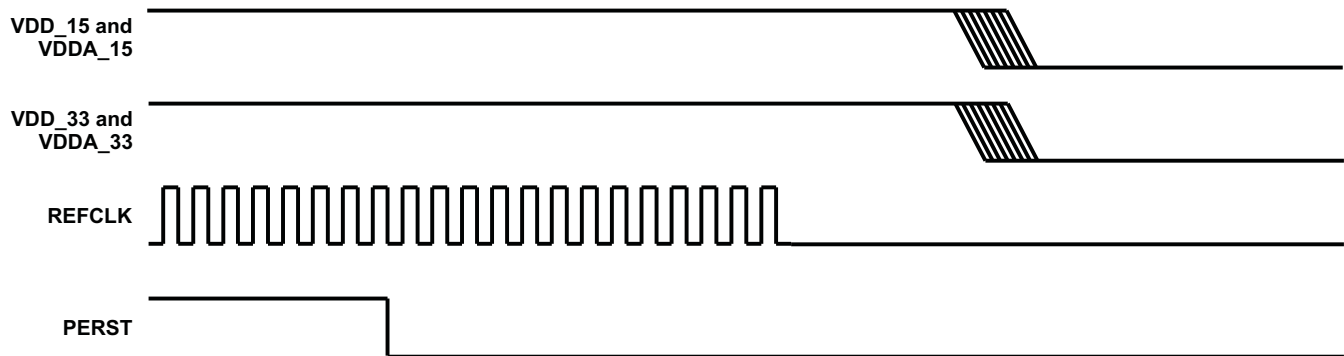
Figure 3-3. Power-Down Sequence
