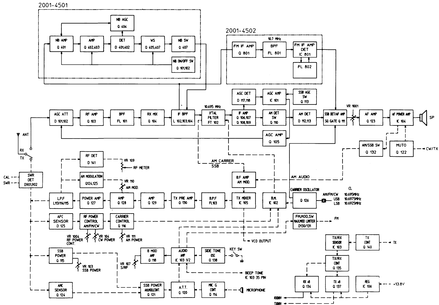
MAIN PCB BLOCK DIAGRAM
