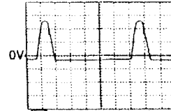
⑫ 50V/cm, 10μs/cm
