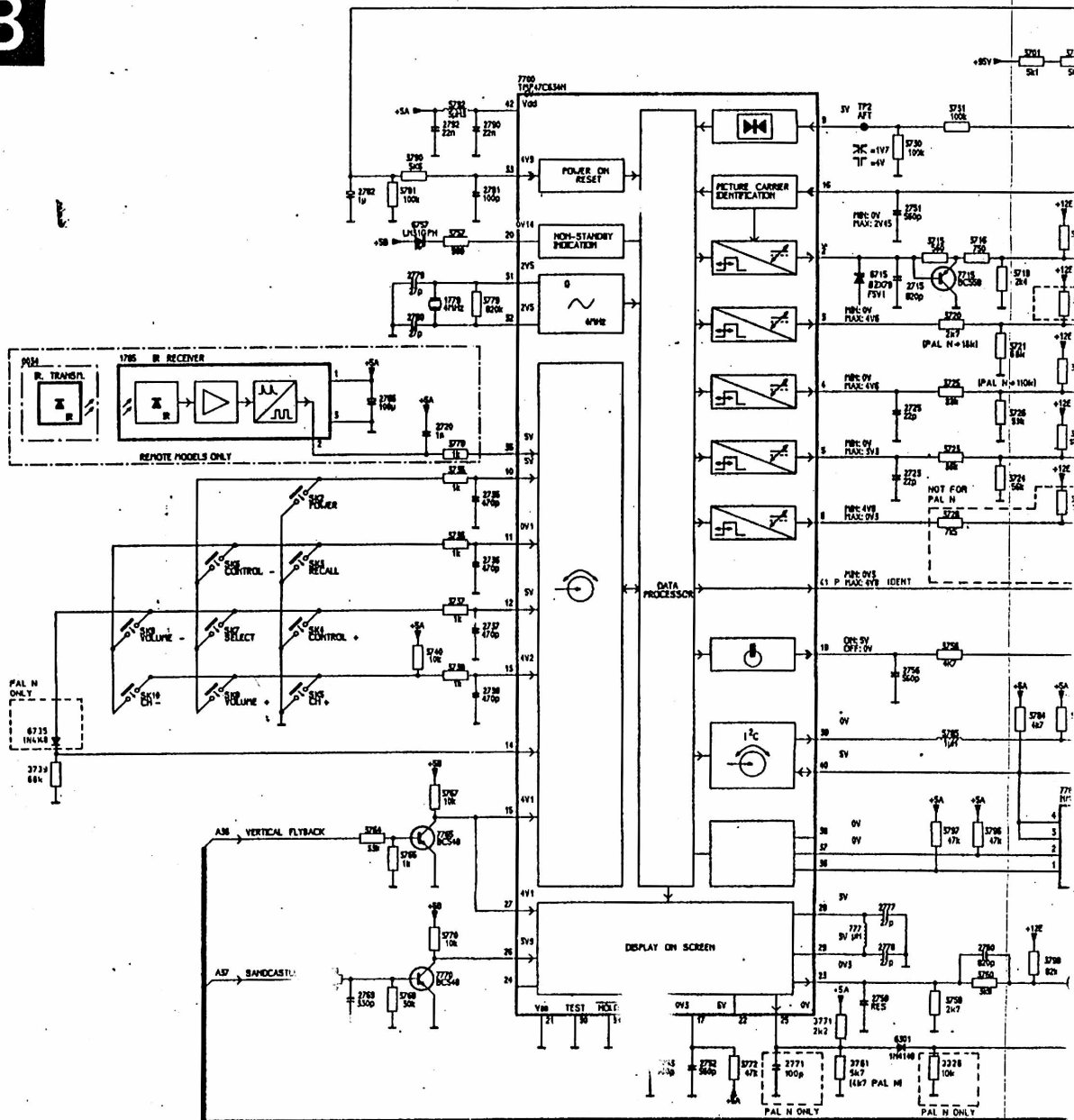
DIAGRAM B (PLL CONTROL)
